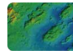
Environmental Research
